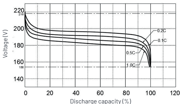
Discharge performance with different rate @ 25°C
